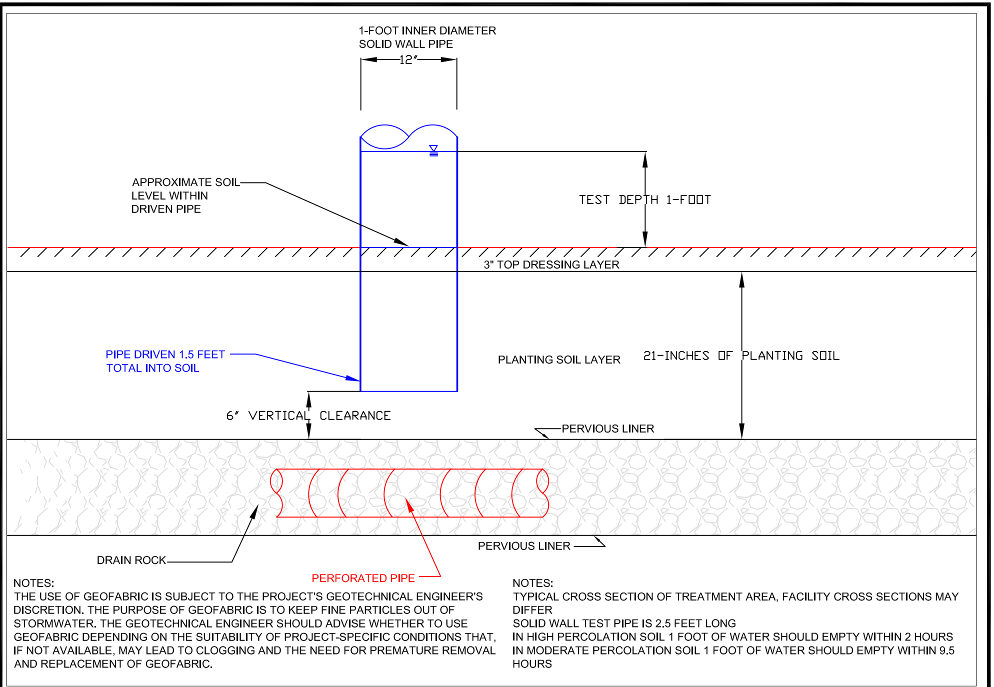
FIGURE 1 PERCOLATION TEST SETUP ACCWP
